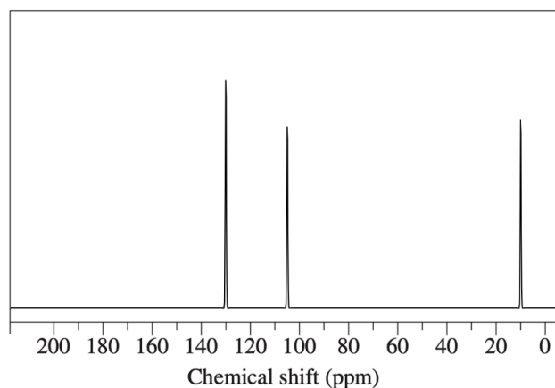
Carbon-13 NMR
